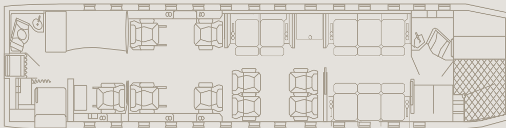
GLOBAL EXPRESS XRS STANDARD CABIN LAYOUT
