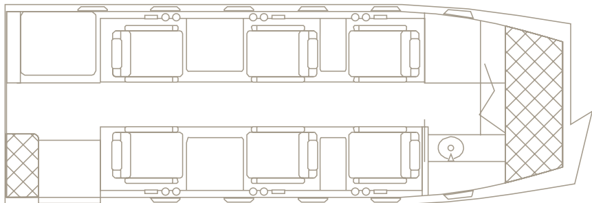
LEARJET 60 STANDARD CABIN CONFIGURATION
